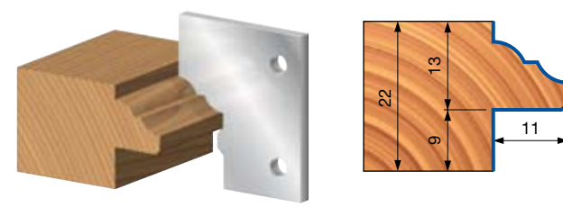
PROFILO / PROFILE 5A
