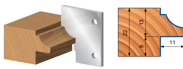
PROFILO / PROFILE 4A
