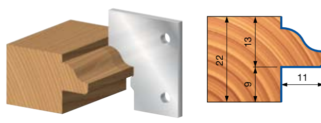
PROFILO / PROFILE 3A
