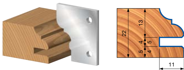
PROFILO / PROFILE 1
